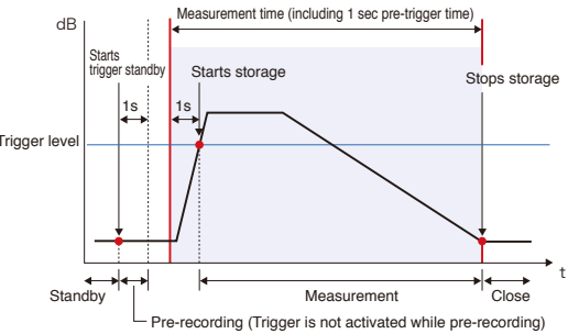
Measurement of reverberation decay curve
