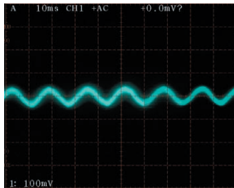
■ Example of waveform measurement using 3471, 60 Hz, 0.1 \mu\text{T} (= 1 mG) (When the tester is connected to an analog oscilloscope.)
