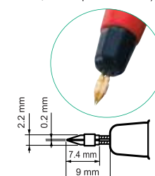
9771 PIN TYPE LEADS (Cable length: connector to fork 40 cm, fork to probes 25 cm)
