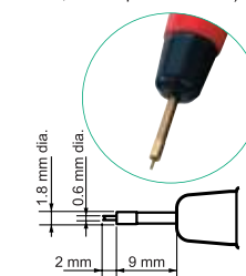
9770 PIN TYPE LEADS (Cable length: connector to fork 40 cm, fork to probes 25 cm)
